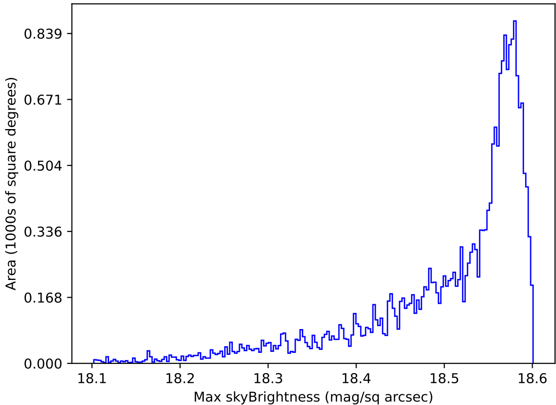
roll_pause_mjdp365_v3.4_10yrs All sky y band: Max skyBrightness
