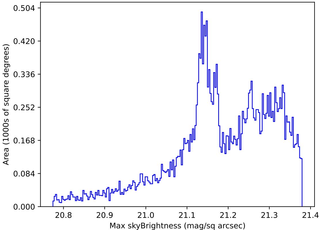
roll_pause_mjdp365_v3.4_10yrs All sky r band: Max skyBrightness
