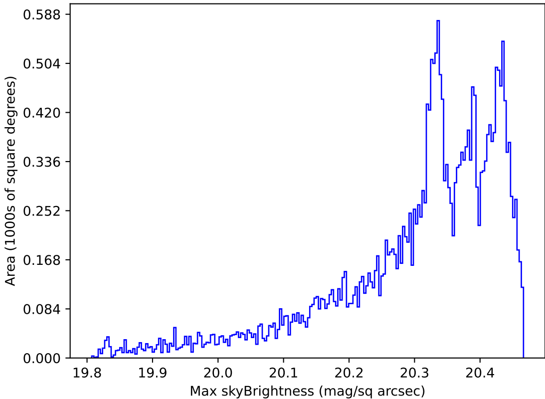
roll_pause_mjdp365_v3.4_10yrs All sky i band: Max skyBrightness
