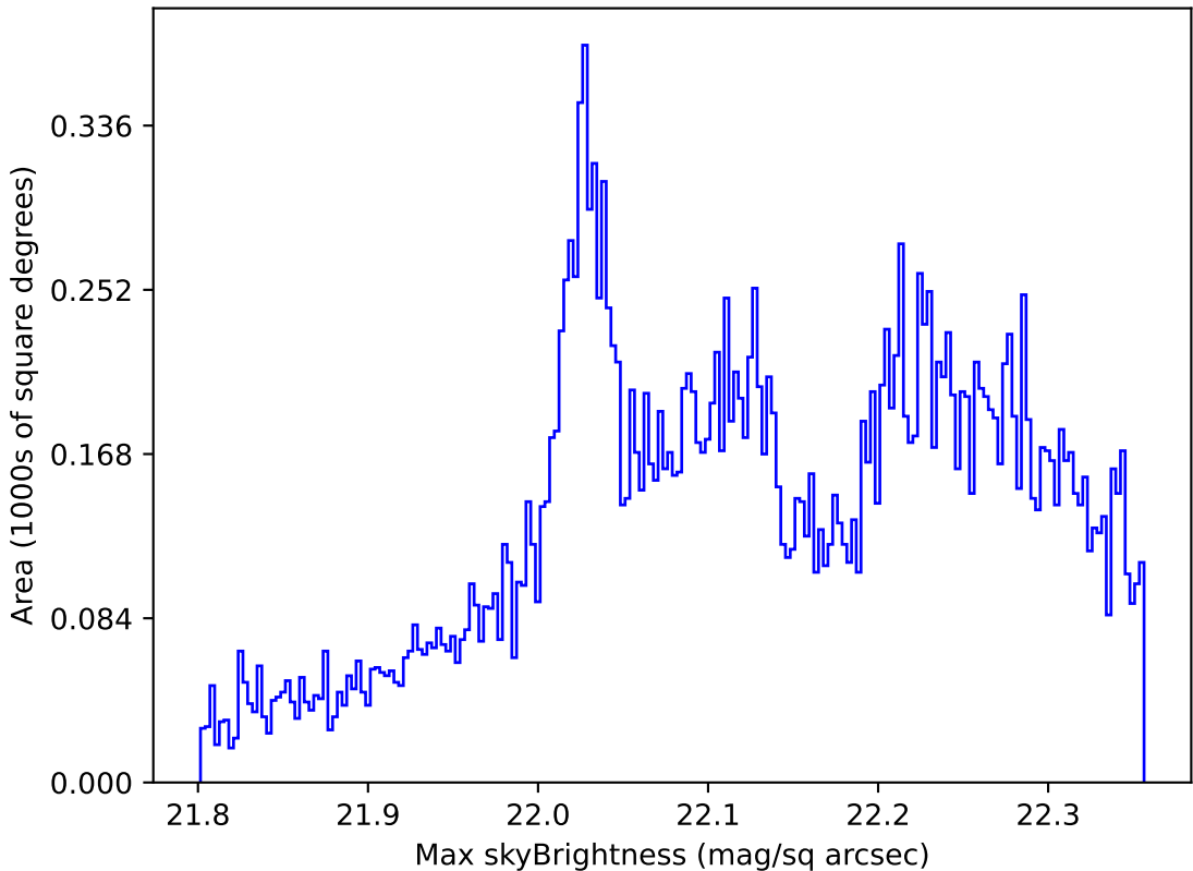
roll_pause_mjdp365_v3.4_10yrs All sky g band: Max skyBrightness
