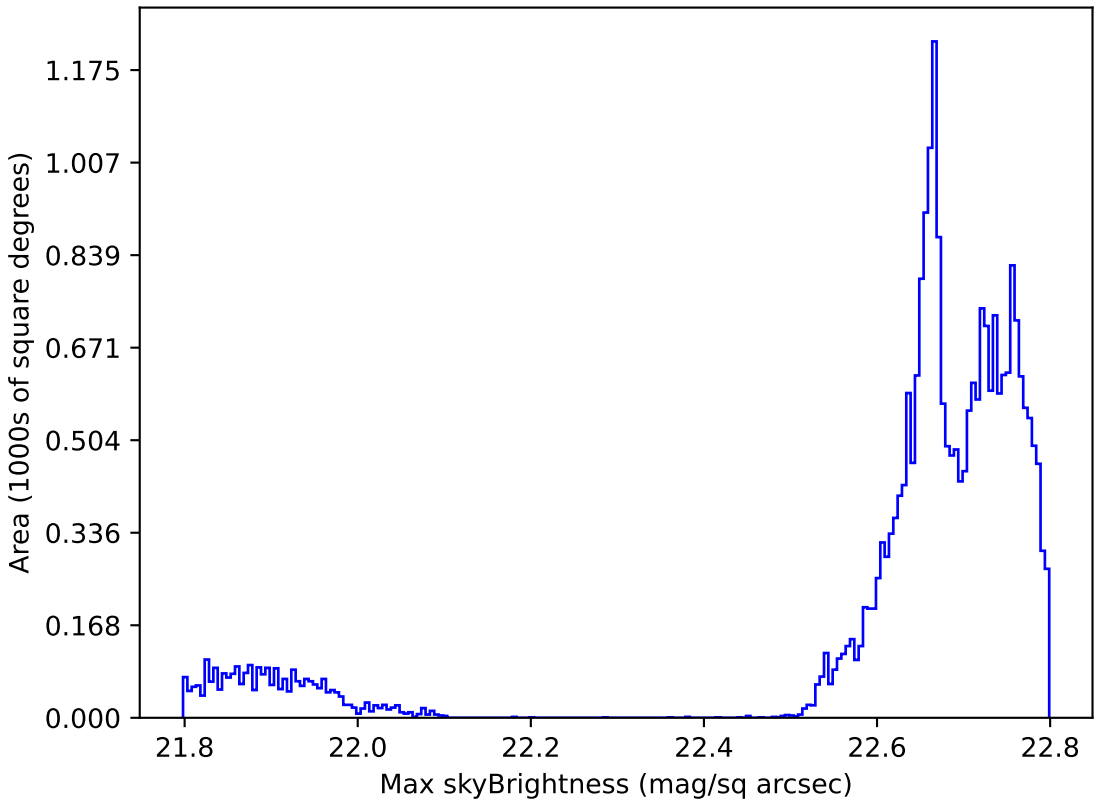
roll_pause_mjdp365_v3.4_10yrs All sky all bands: Max skyBrightness
