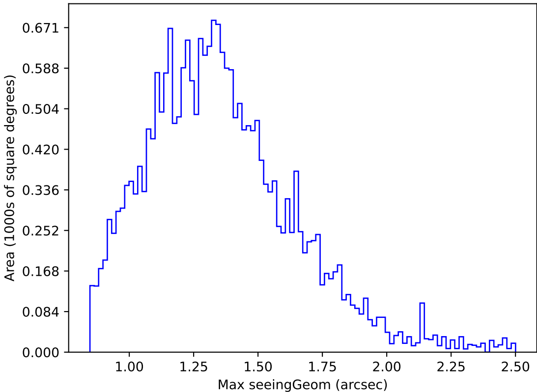
roll_pause_mjdp365_v3.4_10yrs Yr 1 u band: Max seeingGeom
