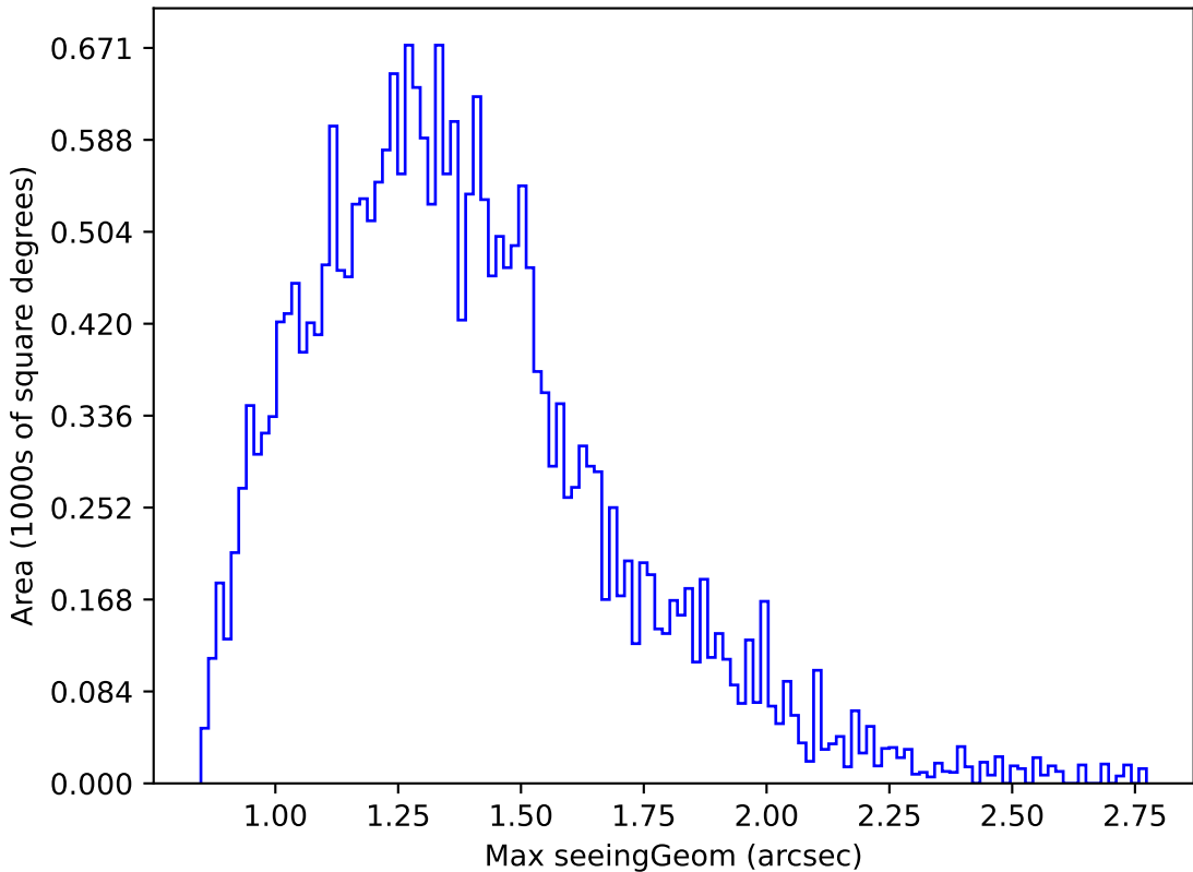
roll_pause_mjdp365_v3.4_10yrs Yr 1 g band: Max seeingGeom
