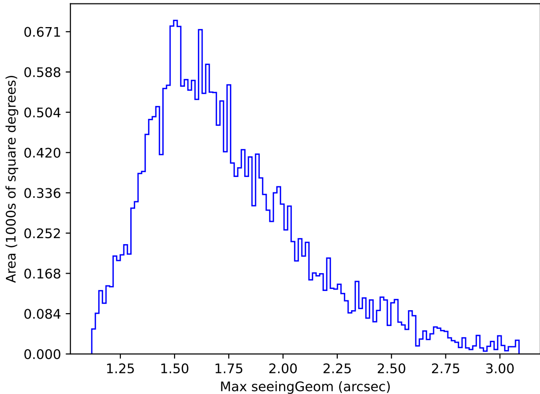
roll_pause_mjdp365_v3.4_10yrs Yr 1 all bands: Max seeingGeom
