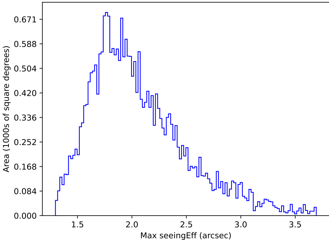
roll_pause_mjdp365_v3.4_10yrs Yr 1 all bands: Max seeingEff
