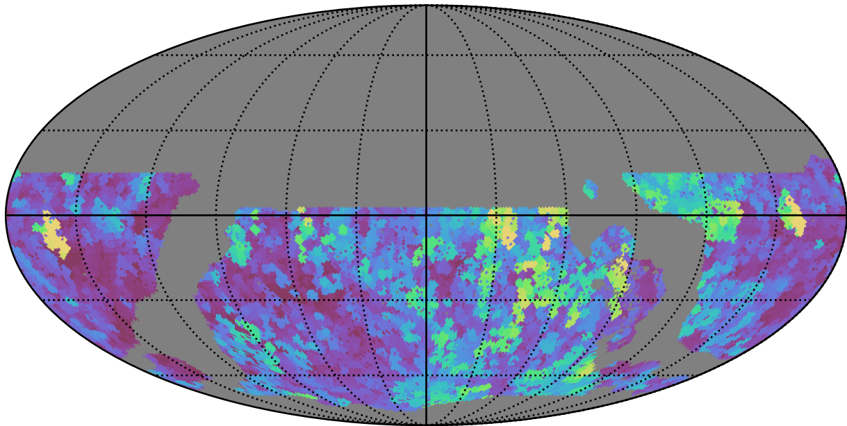
roll_pause_mjdp365_v3.4_10yrs WFD all bands: Max seeingEff
