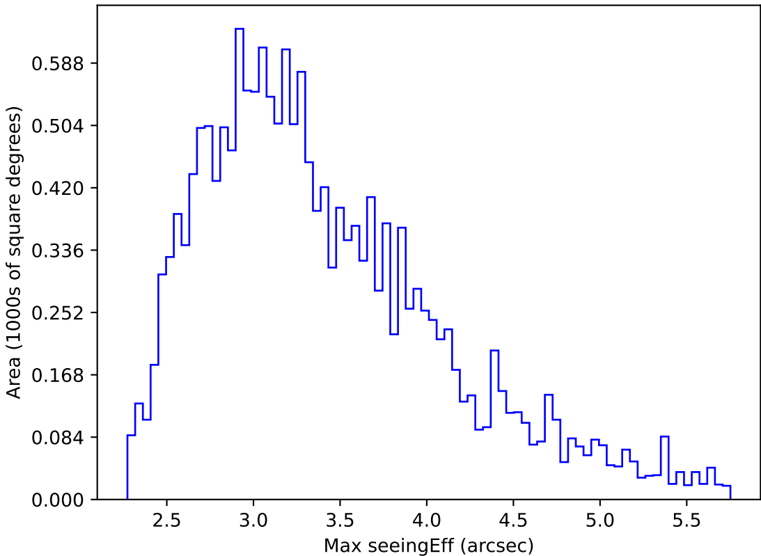
roll_pause_mjdp365_v3.4_10yrs WFD all bands: Max seeingEff
