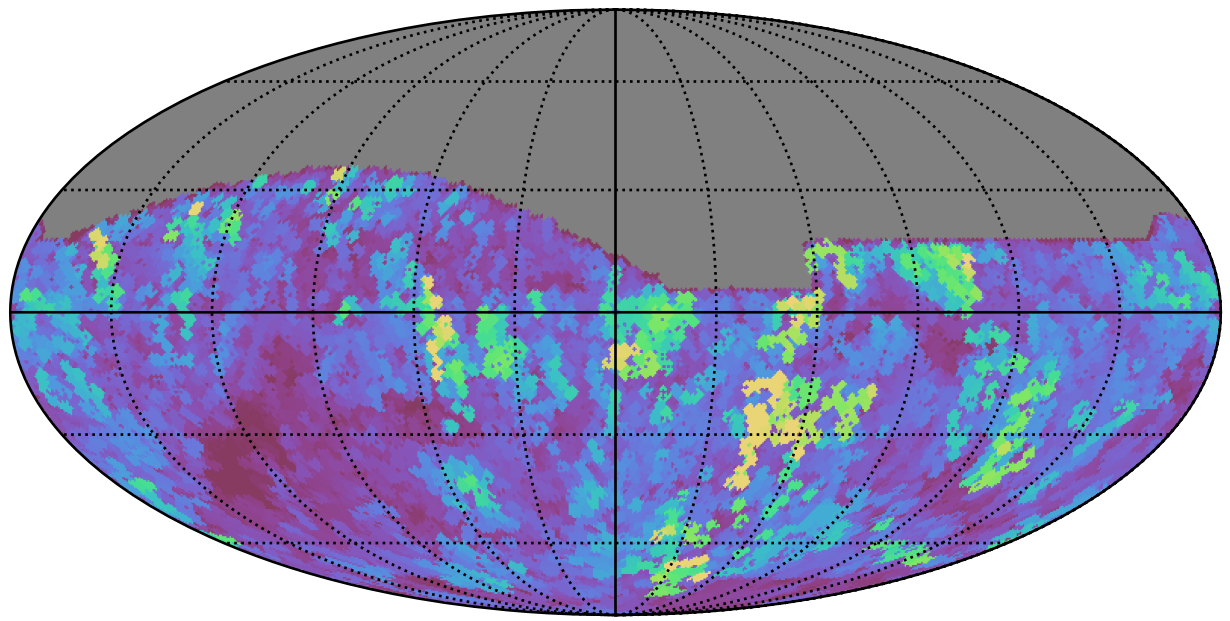
roll_pause_mjdp365_v3.4_10yrs All sky z band: Max seeingEff
