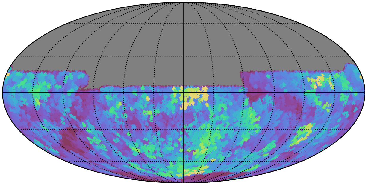
roll_pause_mjdp365_v3.4_10yrs All sky y band: Max seeingEff
