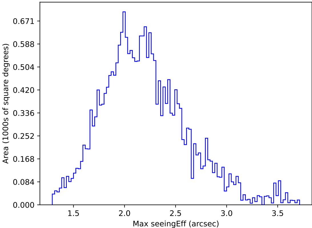
roll_pause_mjdp365_v3.4_10yrs All sky y band: Max seeingEff
