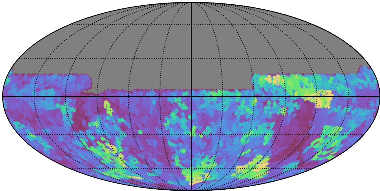
roll_pause_mjdp365_v3.4_10yrs All sky u band: Max seeingEff
