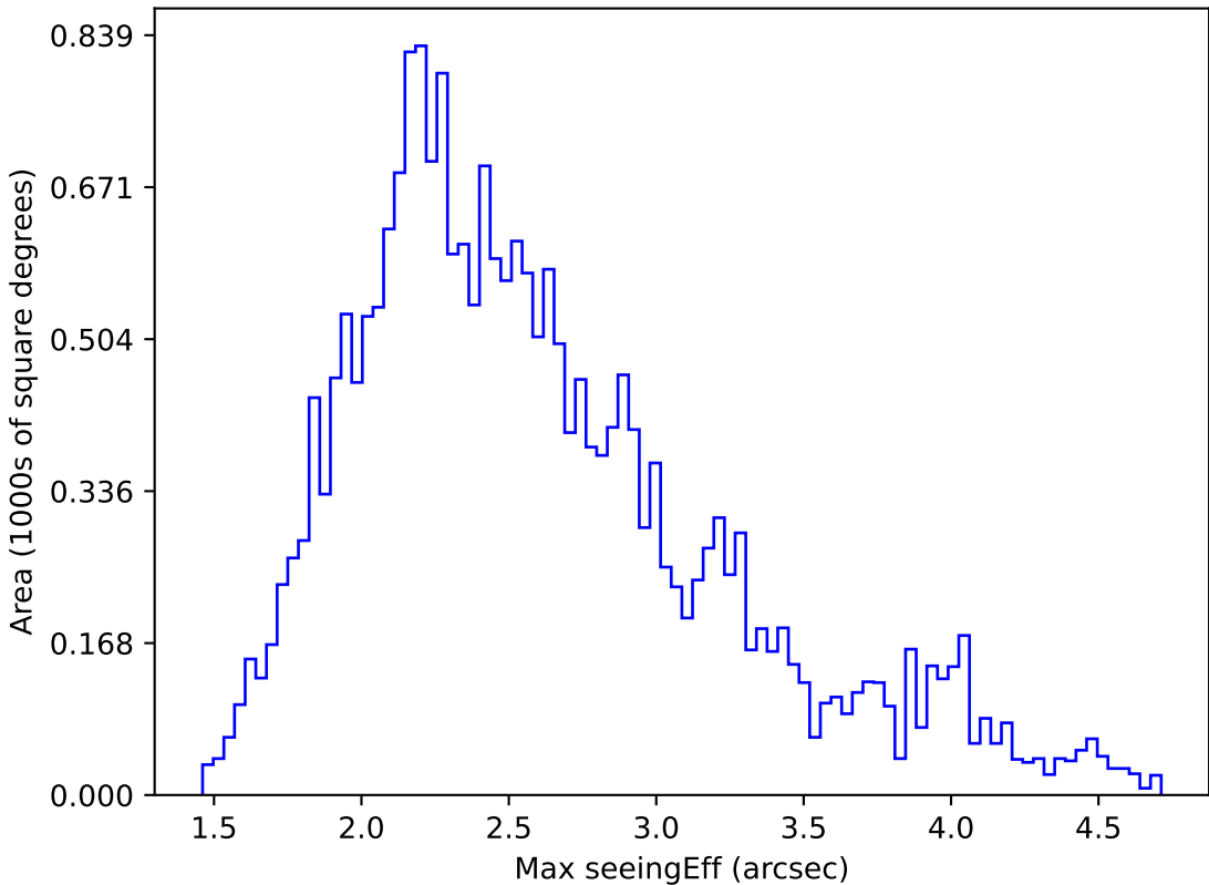
roll_pause_mjdp365_v3.4_10yrs All sky u band: Max seeingEff
