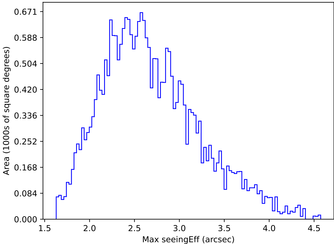
roll_pause_mjdp365_v3.4_10yrs All sky r band: Max seeingEff
