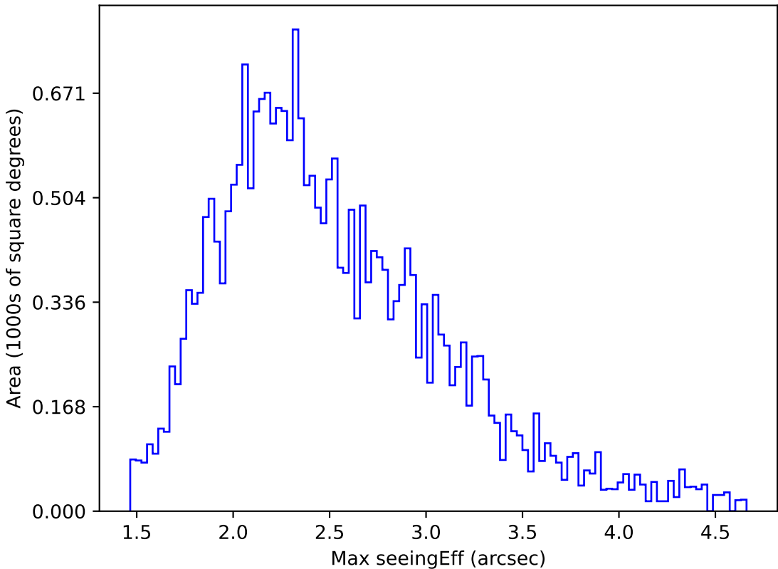
roll_pause_mjdp365_v3.4_10yrs All sky g band: Max seeingEff
