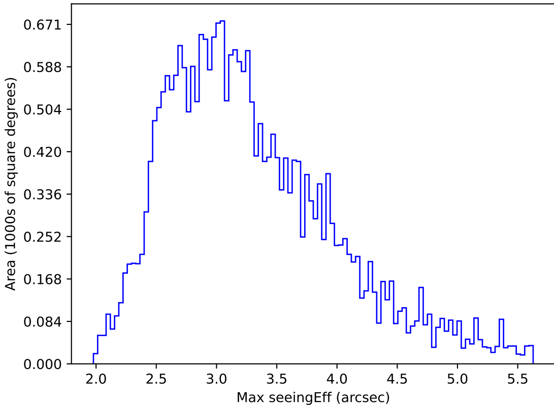
roll_pause_mjdp365_v3.4_10yrs All sky all bands: Max seeingEff
