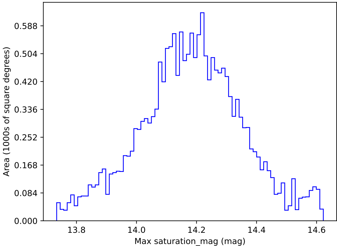
roll_pause_mjdp365_v3.4_10yrs WFD y band: Max saturation_mag
