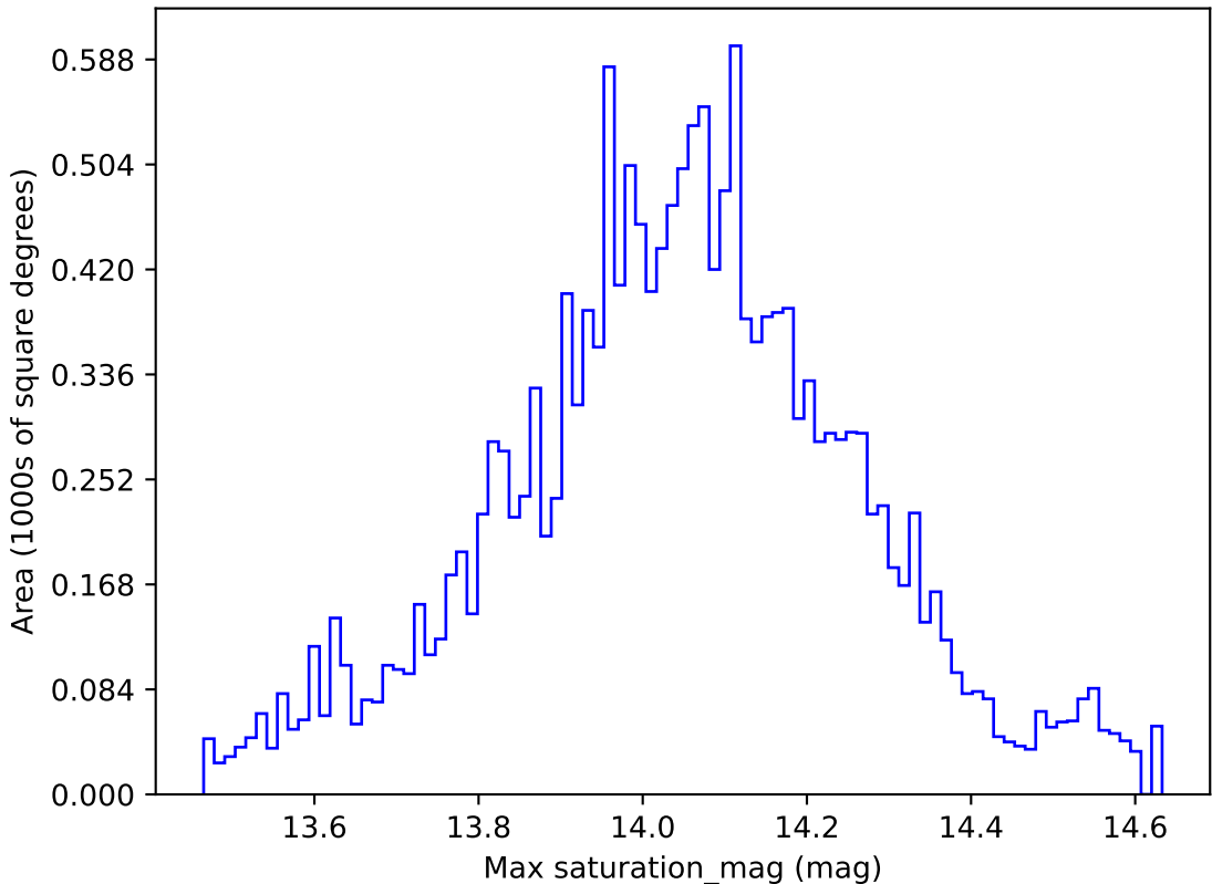
roll_pause_mjdp365_v3.4_10yrs WFD u band: Max saturation_mag
