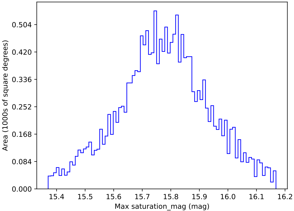
roll_pause_mjdp365_v3.4_10yrs WFD r band: Max saturation_mag
