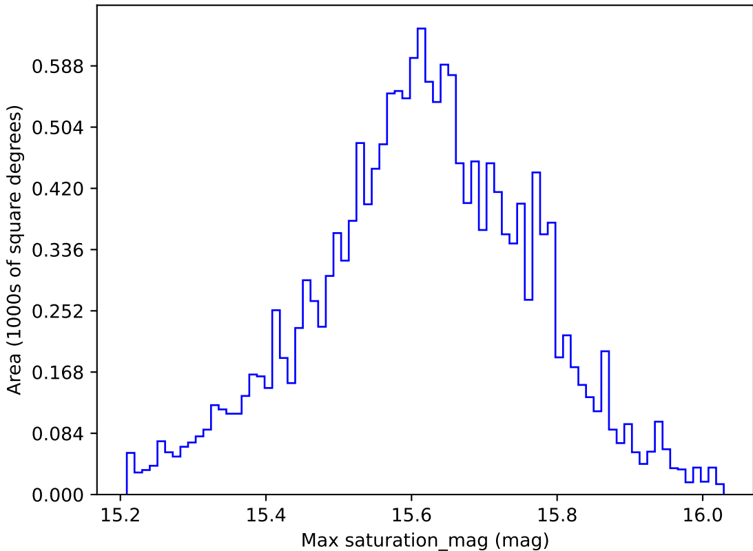
roll_pause_mjdp365_v3.4_10yrs WFD i band: Max saturation_mag
