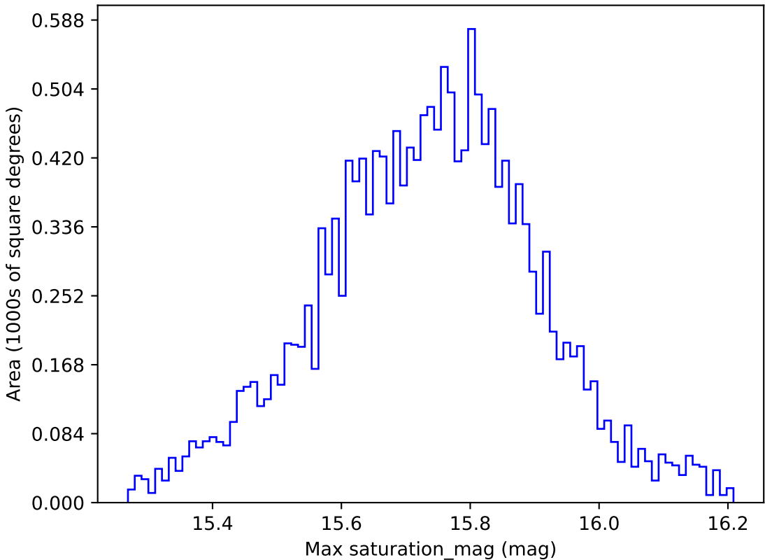
roll_pause_mjdp365_v3.4_10yrs WFD g band: Max saturation_mag
