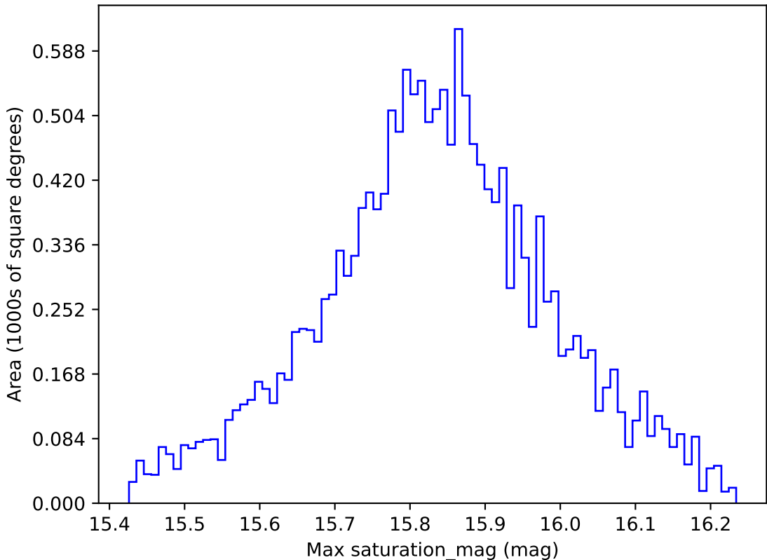
roll_pause_mjdp365_v3.4_10yrs WFD all bands: Max saturation_mag
