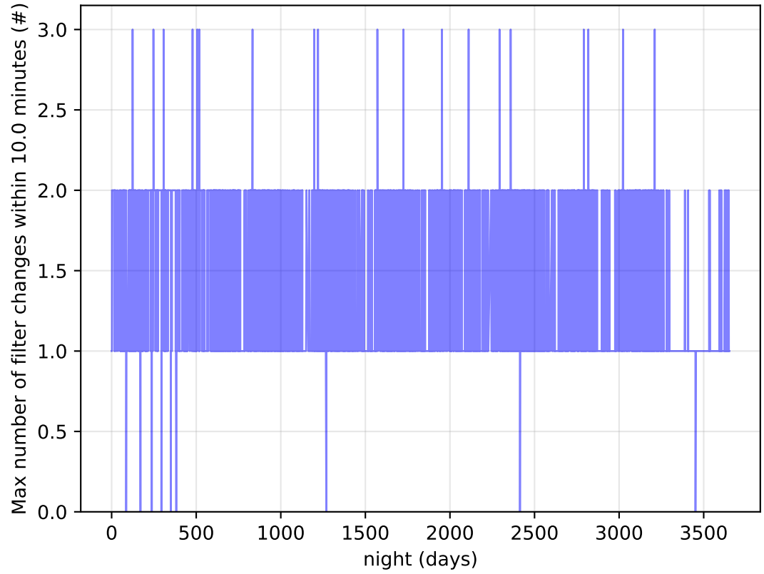
roll_pause_mjdp365_v3.4_10yrs Per Night: Max number of filter changes within 10.0 minutes
