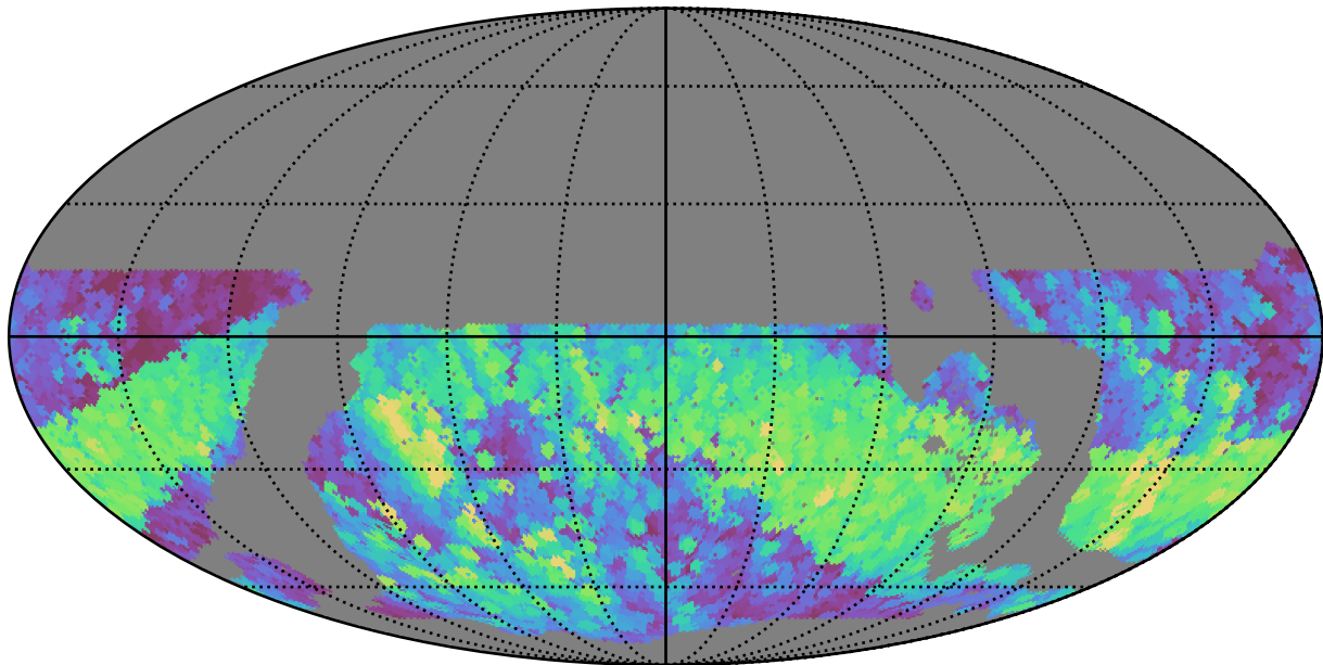
roll_pause_mjdp365_v3.4_10yrs WFD r band: Max normairmass
