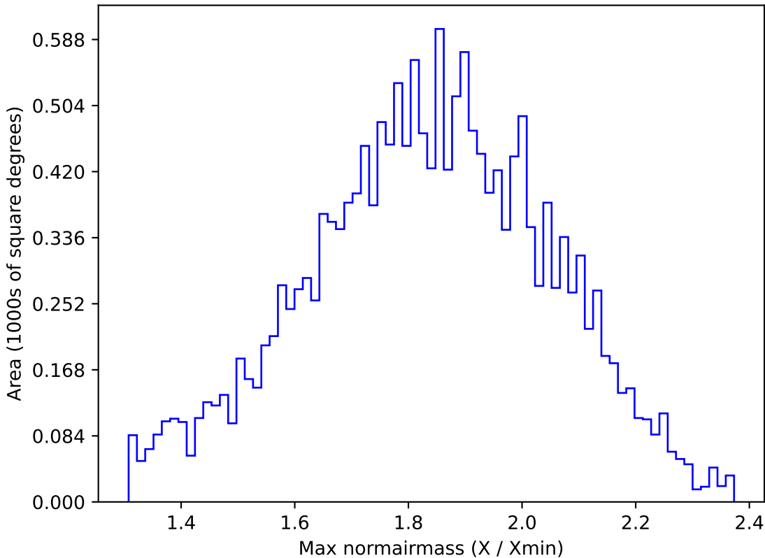
roll_pause_mjdp365_v3.4_10yrs WFD g band: Max normairmass
