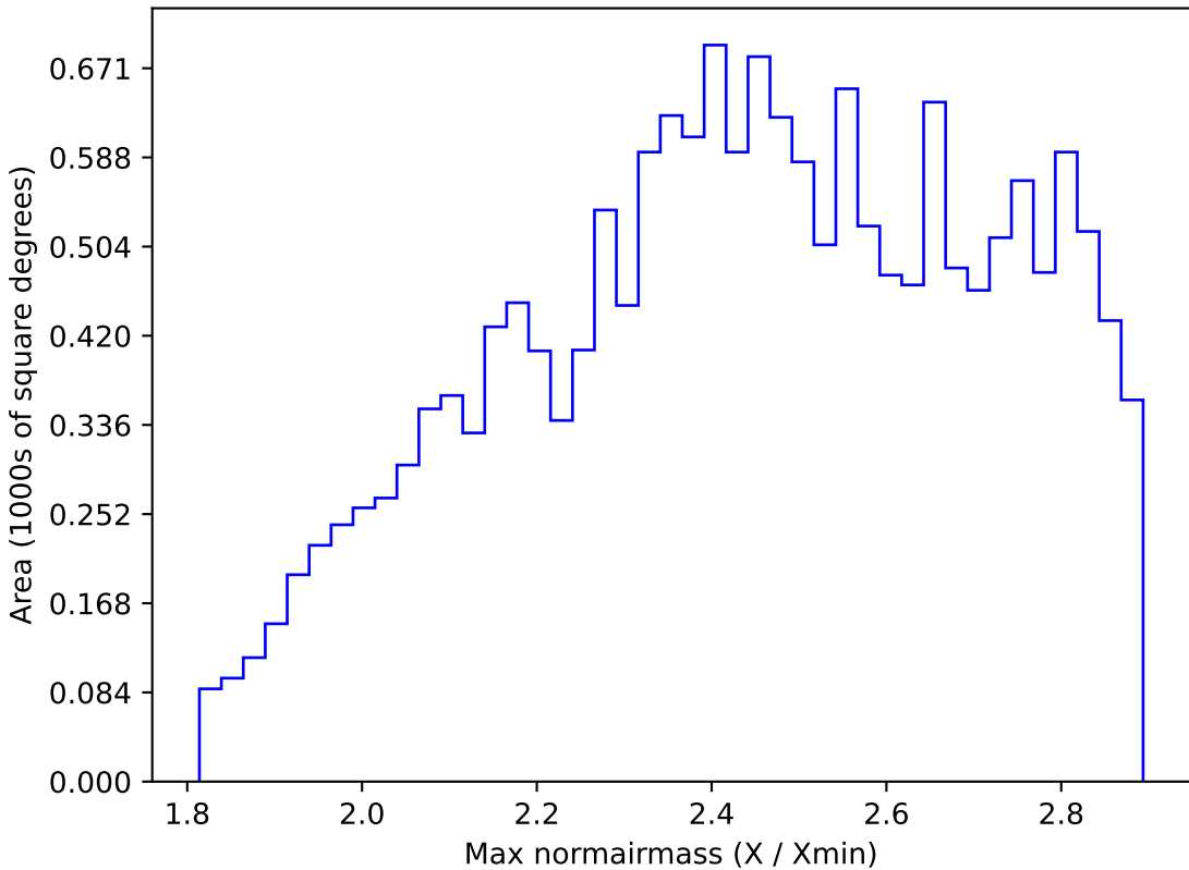
roll_pause_mjdp365_v3.4_10yrs WFD all bands: Max normairmass
