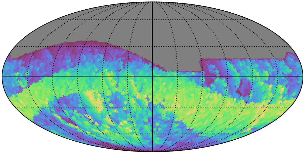
roll_pause_mjdp365_v3.4_10yrs All sky r band: Max normairmass
