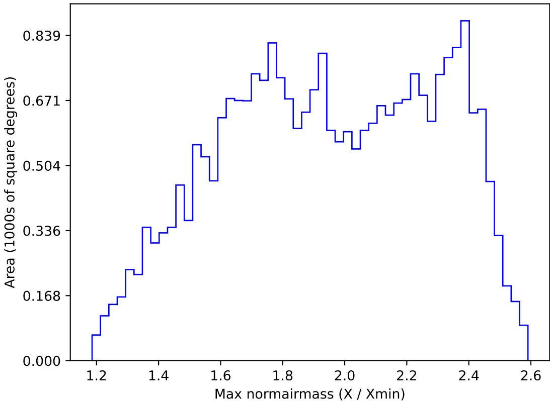
roll_pause_mjdp365_v3.4_10yrs All sky r band: Max normairmass
