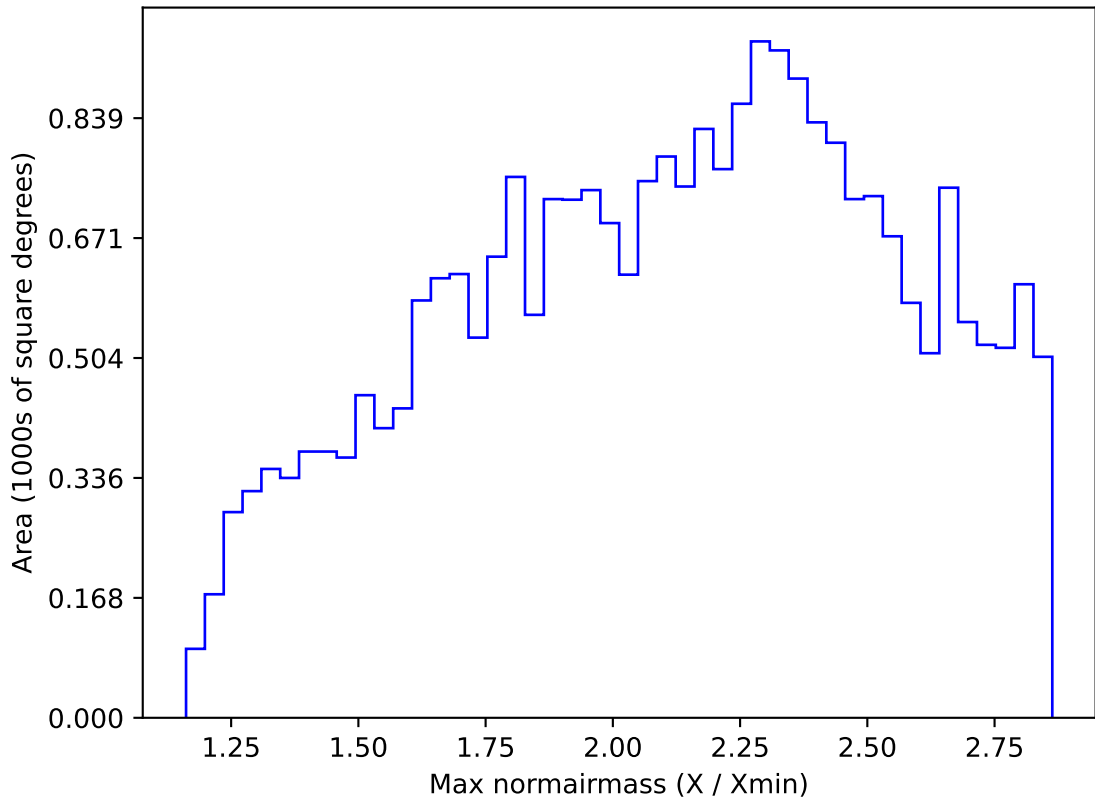
roll_pause_mjdp365_v3.4_10yrs All sky i band: Max normairmass
