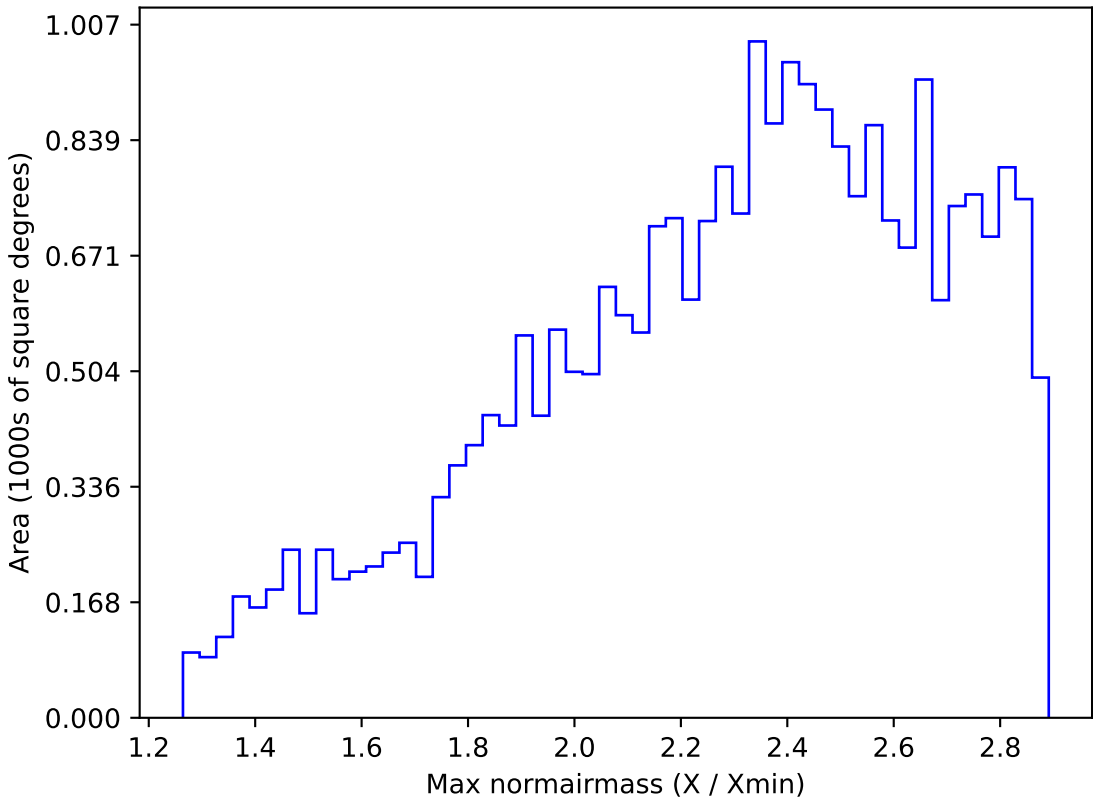
roll_pause_mjdp365_v3.4_10yrs All sky all bands: Max normairmass
