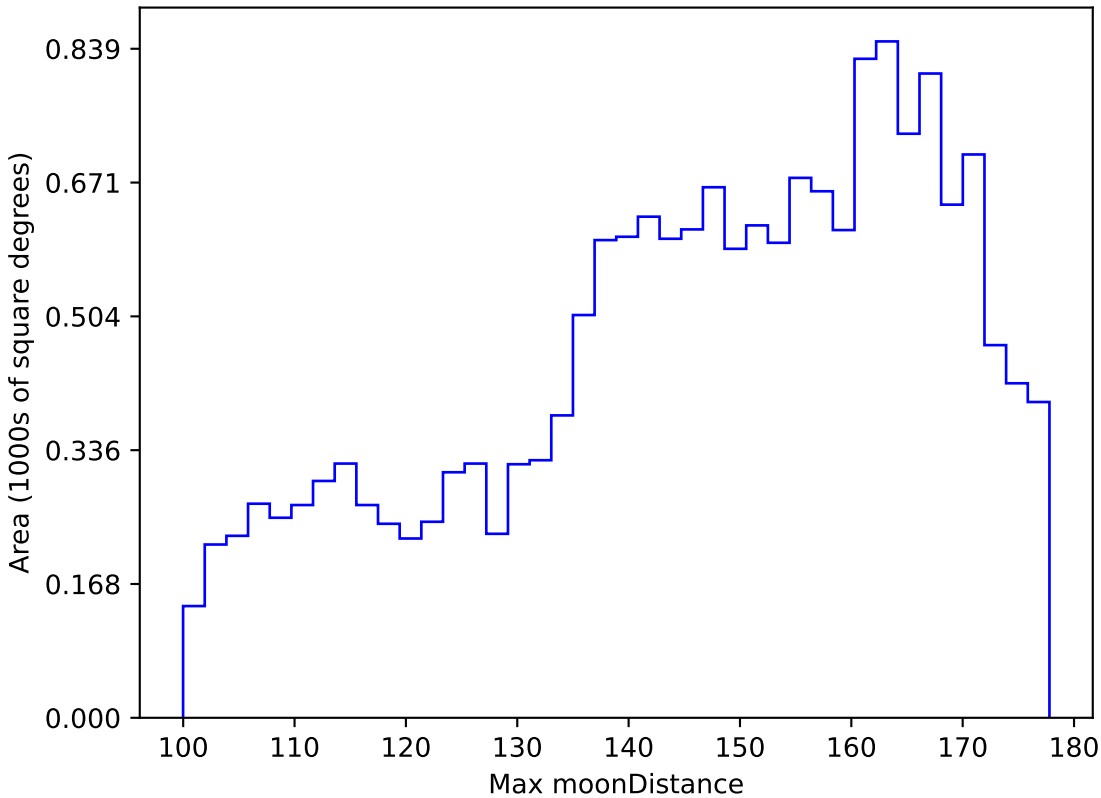
roll_pause_mjdp365_v3.4_10yrs WFD y band: Max moonDistance
