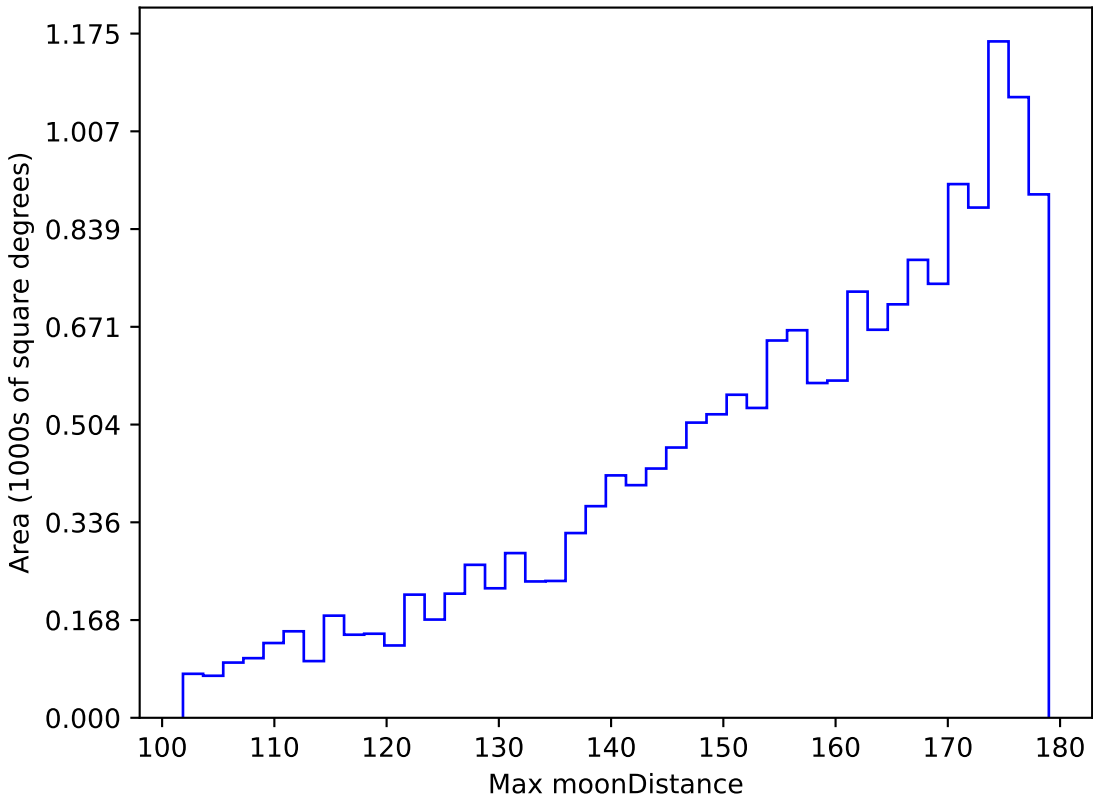
roll_pause_mjdp365_v3.4_10yrs WFD u band: Max moonDistance
