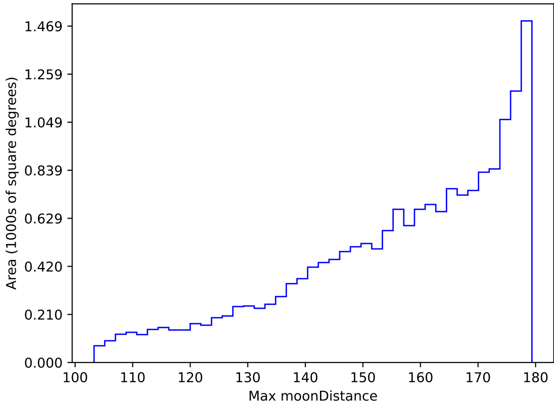
roll_pause_mjdp365_v3.4_10yrs WFD r band: Max moonDistance
