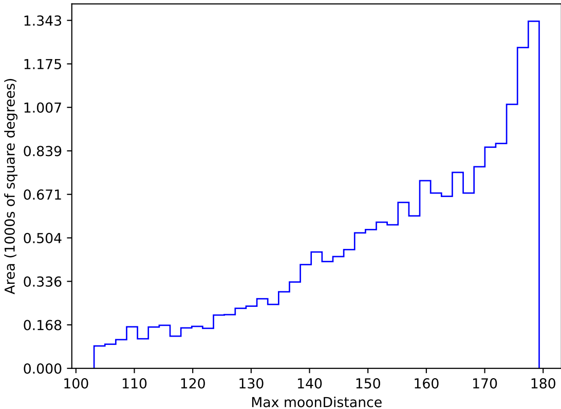
roll_pause_mjdp365_v3.4_10yrs WFD i band: Max moonDistance
