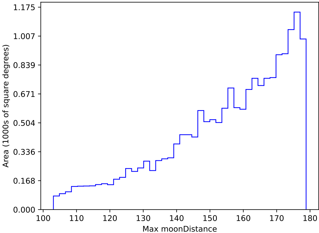
roll_pause_mjdp365_v3.4_10yrs WFD g band: Max moonDistance
