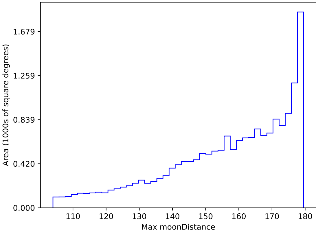
roll_pause_mjdp365_v3.4_10yrs WFD all bands: Max moonDistance
