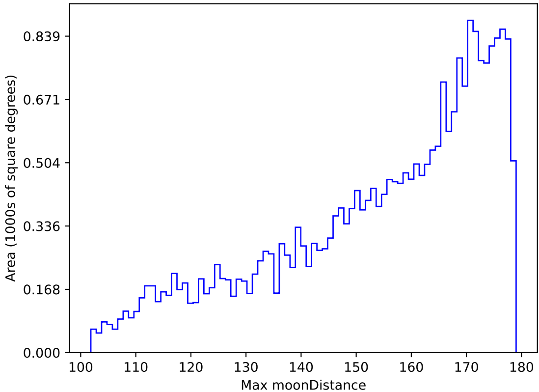
roll_pause_mjdp365_v3.4_10yrs All sky z band: Max moonDistance
