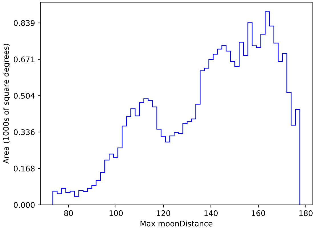
roll_pause_mjdp365_v3.4_10yrs All sky y band: Max moonDistance
