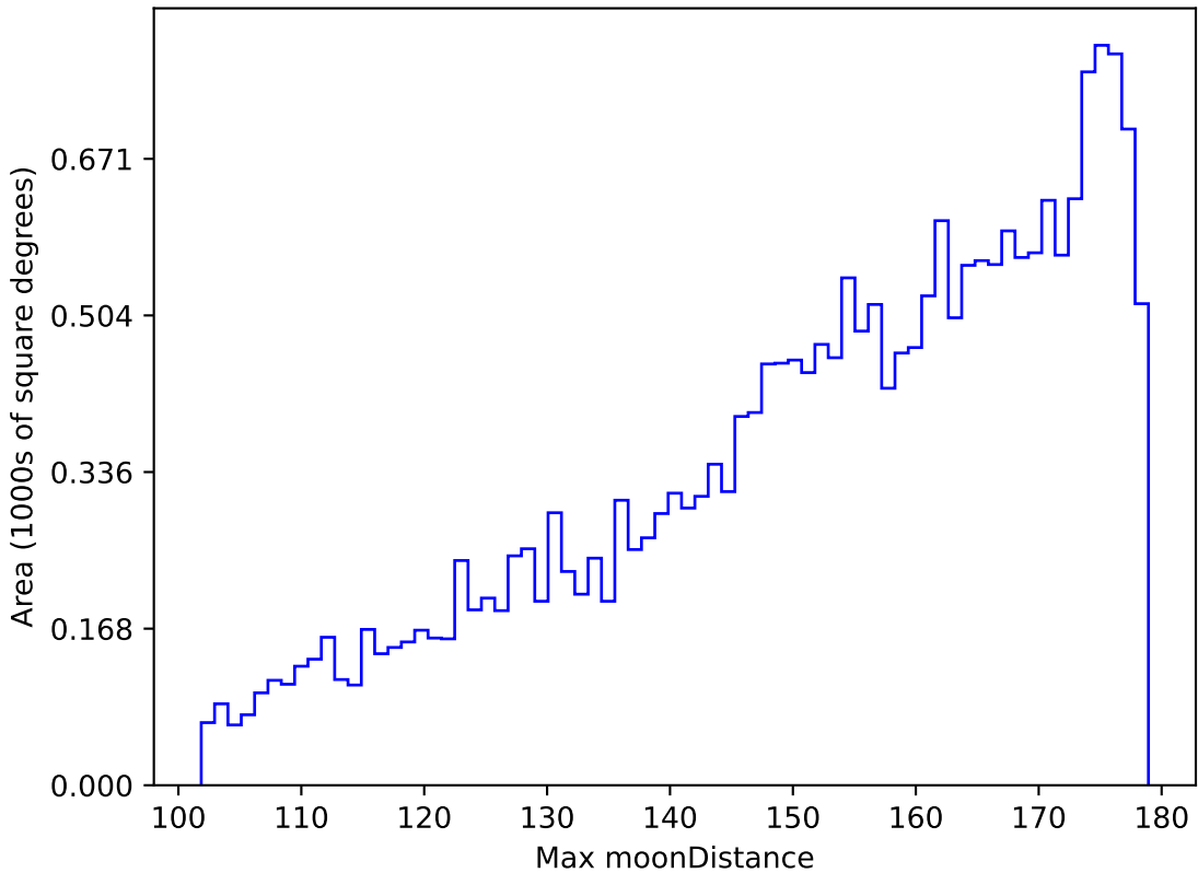
roll_pause_mjdp365_v3.4_10yrs All sky u band: Max moonDistance
