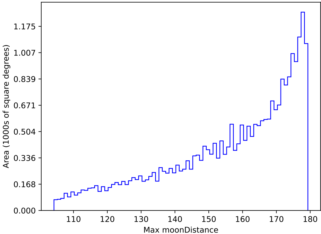
roll_pause_mjdp365_v3.4_10yrs All sky r band: Max moonDistance
