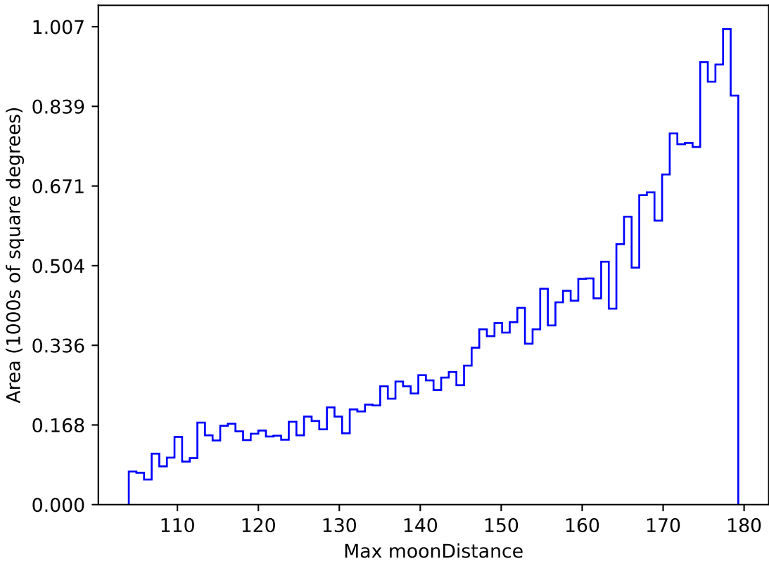
roll_pause_mjdp365_v3.4_10yrs All sky i band: Max moonDistance
