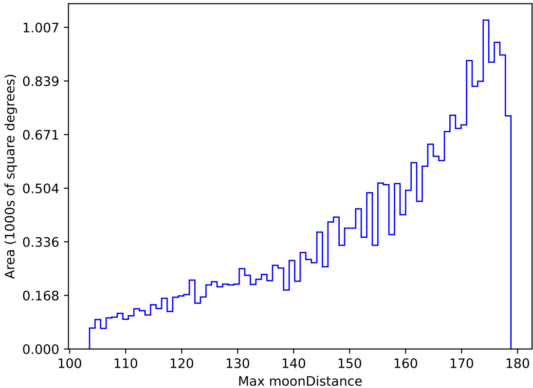
roll_pause_mjdp365_v3.4_10yrs All sky g band: Max moonDistance
