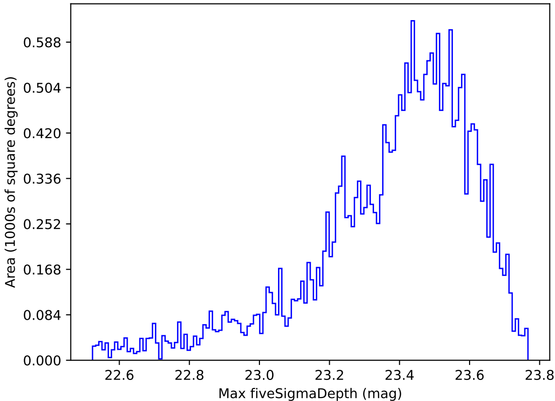
roll_pause_mjdp365_v3.4_10yrs Yr 1 z band: Max fiveSigmaDepth
