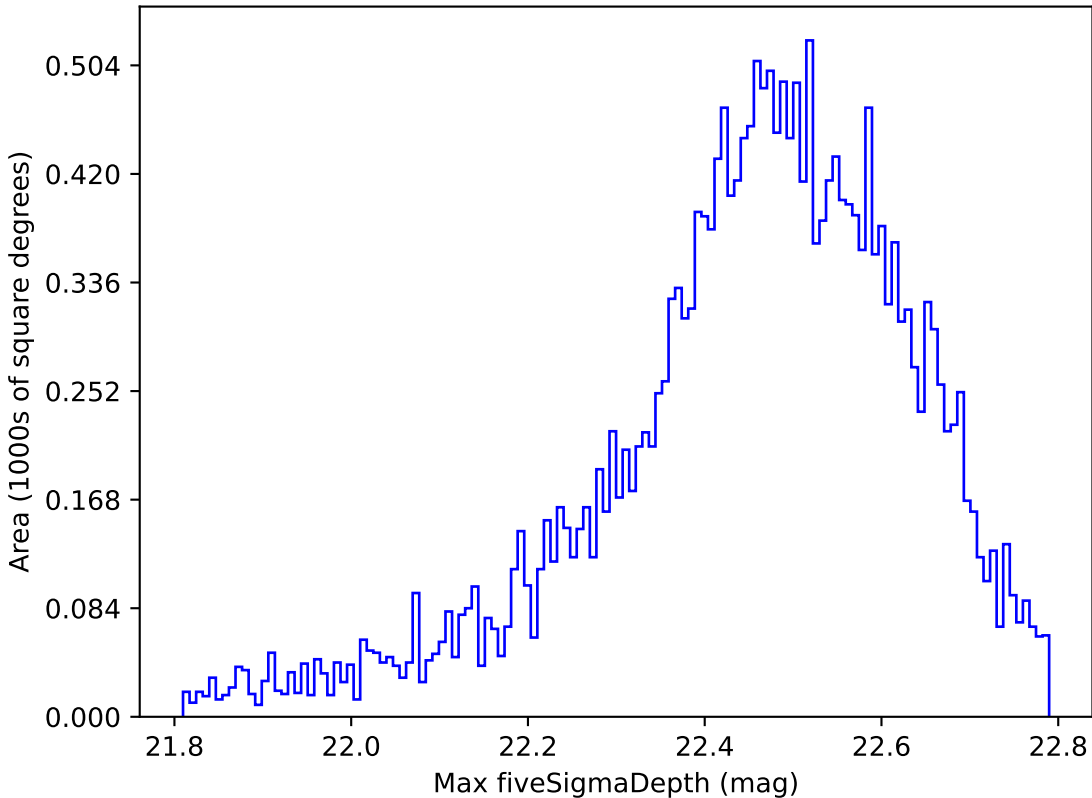
roll_pause_mjdp365_v3.4_10yrs Yr 1 y band: Max fiveSigmaDepth
