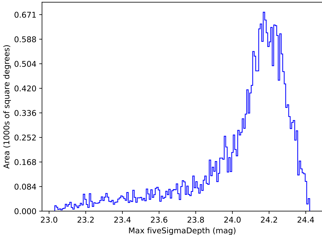
roll_pause_mjdp365_v3.4_10yrs Yr 1 i band: Max fiveSigmaDepth
