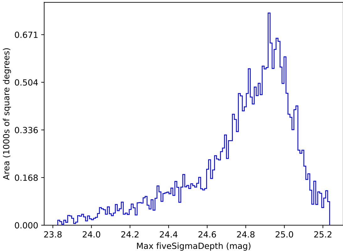
roll_pause_mjdp365_v3.4_10yrs Yr 1 g band: Max fiveSigmaDepth
