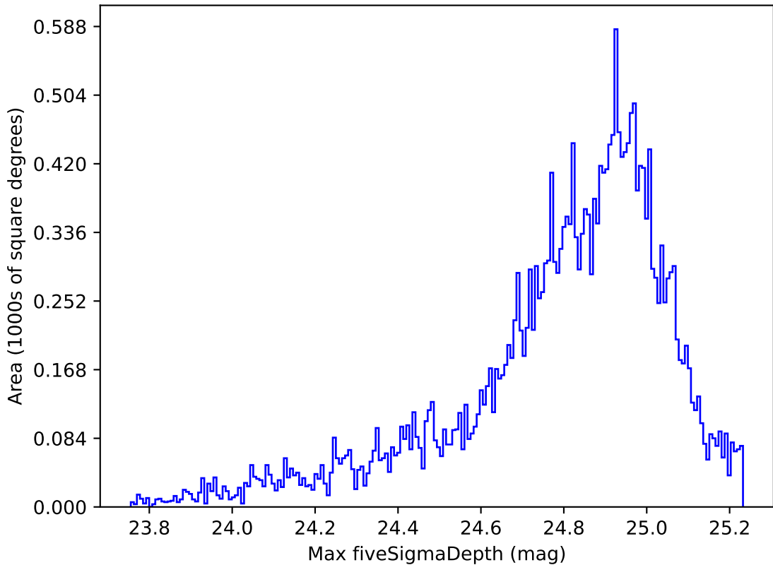
roll_pause_mjdp365_v3.4_10yrs Yr 1 all bands: Max fiveSigmaDepth
